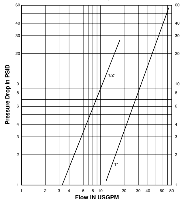
PF Series Performance Flow Data Test Fluid: Water, Body Size: 1/2", 1"
