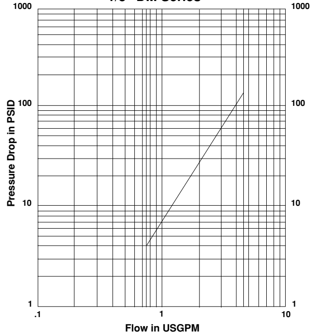
Water Pressure Drop 1/8" DM Series
