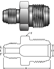
Double Male Reducing Union
