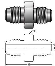
Double Male Union
