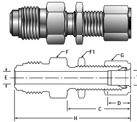
Compression Tube Fitting Bulkhead Connector (A-LOK®)
