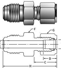
Compression Tube Fitting Connector (A-LOK®)
